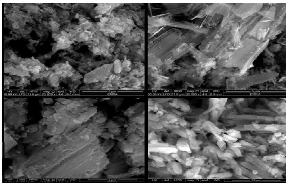
Figure 5. SEM images of \text{TiO}_2 nano powders calcined at 1000 °C prepared from a) methanol, b) isopropanol, and c) isobutyl alcohol
