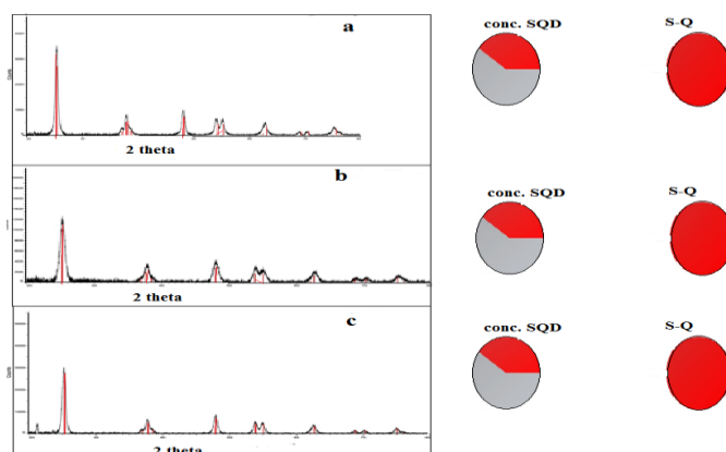
Figure 2. The XRD pattern, a) SQD conc., S-Q for TiO_2 nanoparticles prepared, b) methanol, and c) isopropanol, isobutyl alcohol calcined at 400 °C
