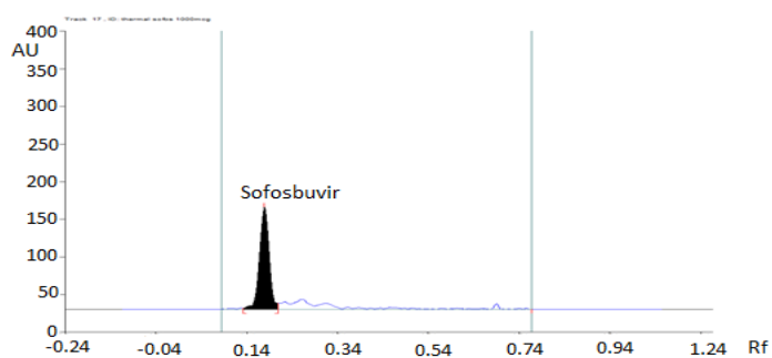
Fig. 4f. Chromatogram of thermal degradation of Sofosbuvir.
