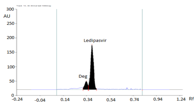
Fig. 3e. Chromatogram of photolytic degradation of ledipasvir
