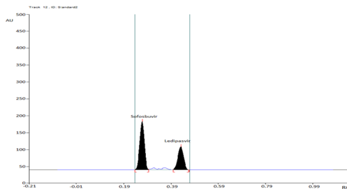
Fig. 6. Chromatogram of formulation (Ledipasvir & Sofosbuvir)
