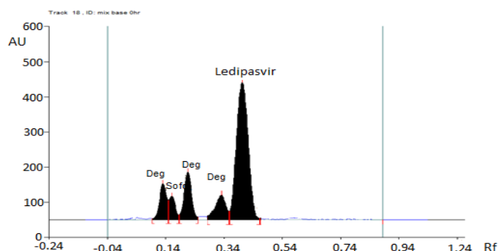
Fig. 5. Chromatogram of stress treated mixture of Ledipasvir and Sofosbuvir.
