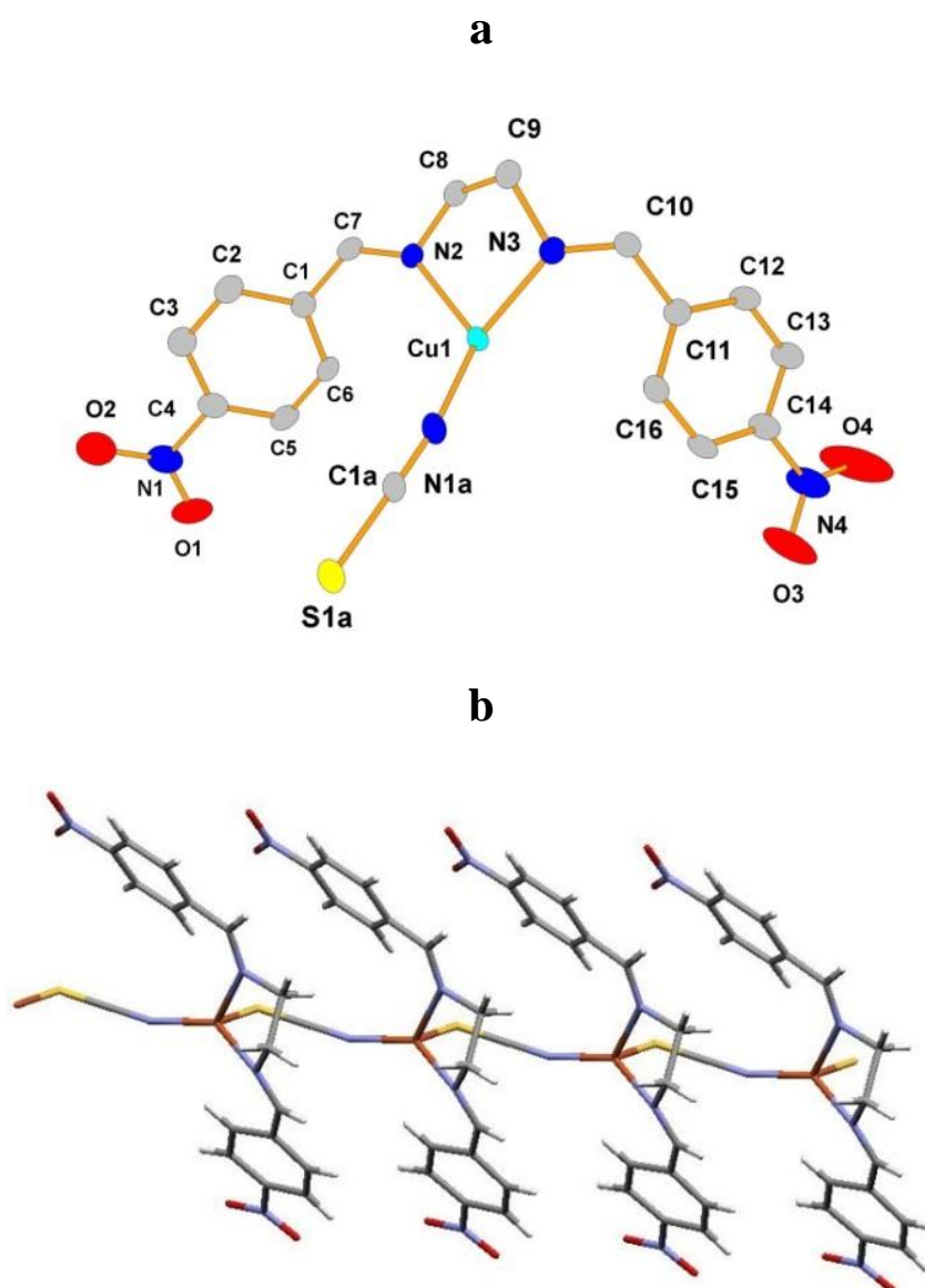
Fig. 4. The crystal structures of maker unit (a) and 1D coordination polymer of 1 (b).
